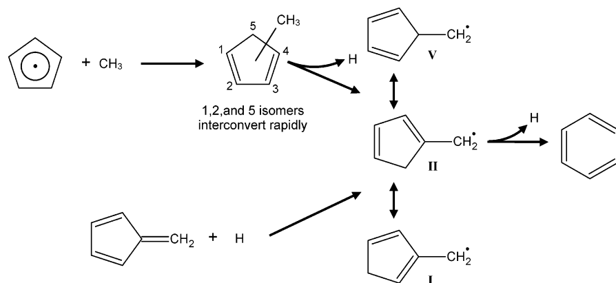
Figure 1. Ring-expansion reactions of cyclopentadienyl systems.
